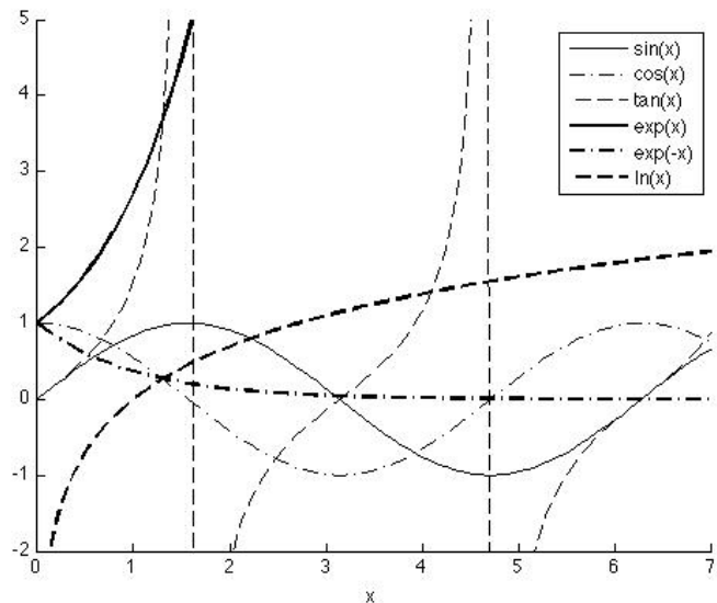
Figure 1: A plot of a few mathematical functions.
